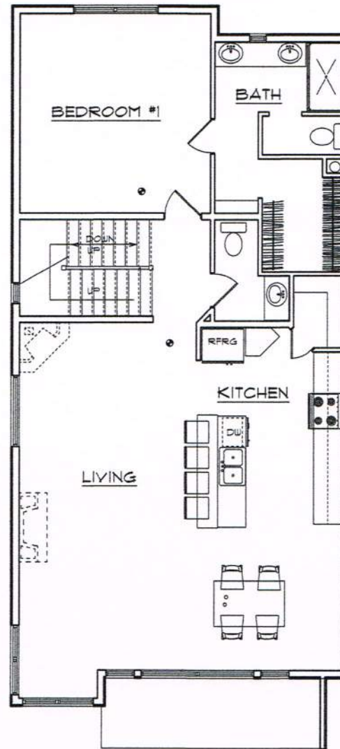
2ND FLOOR LAYOUT
