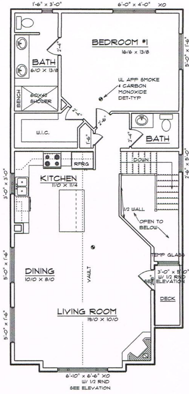
2ND FLOOR LAYOUT SCALE: 1/8" = 1'-0"
