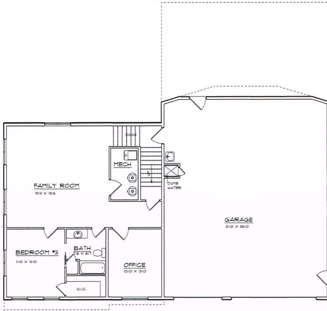
1ST FLOOR LAYOUT
